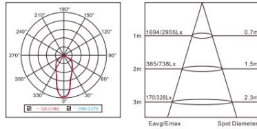
40W 40°
