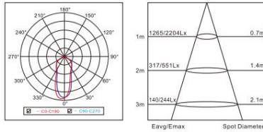
30W 40°
