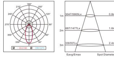
50W 40°
