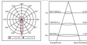
40W 40°
